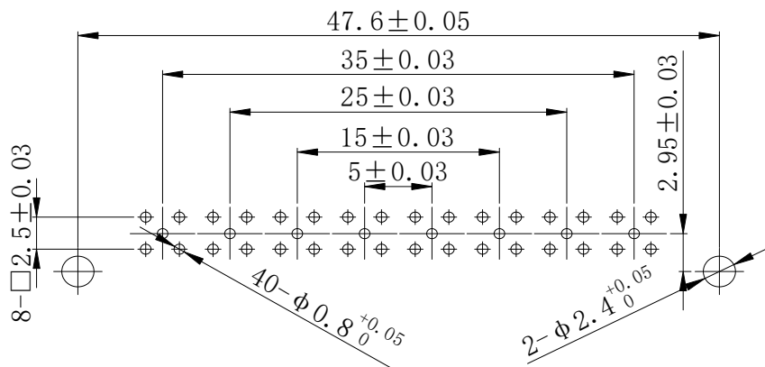
PCB Layout
